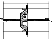
BLOCKAID - BAACL190 SCALE 1:10
