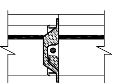
BLOCKAID - BANCL190 SCALE 1:10
