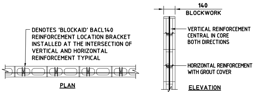
BLOCKAID - BA CL140 SCALE 1:20
