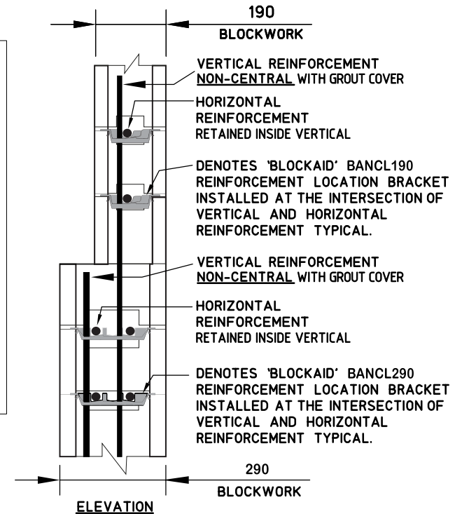
BLOCKAID BA NCL190 & BA NCL290 SCALE 1:10
