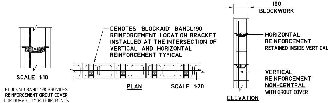
BLOCKAID - BA NCL190
