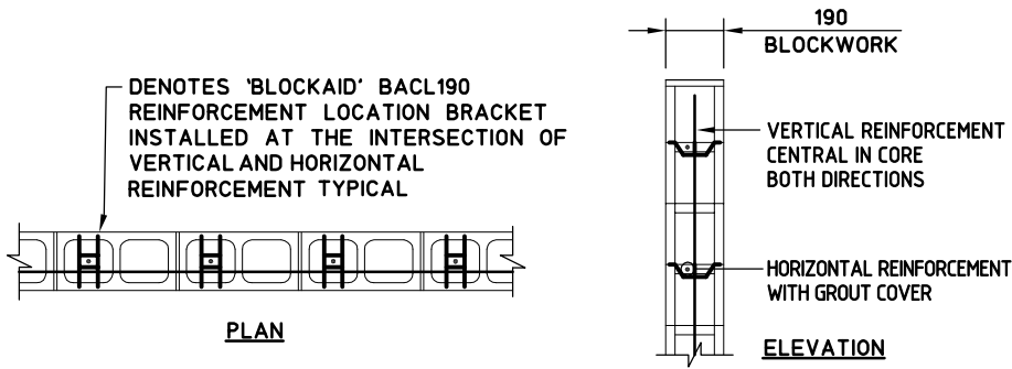
BLOCKAID - BA CL190 SCALE 1:20
